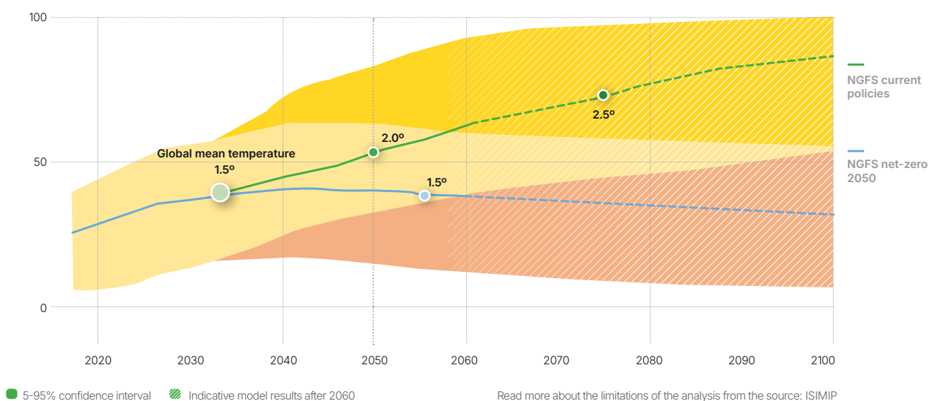
Figure 2. Change in the proportion of areas exposed to severe drought in Türkiye under different scenarios (SPEI < -2)
