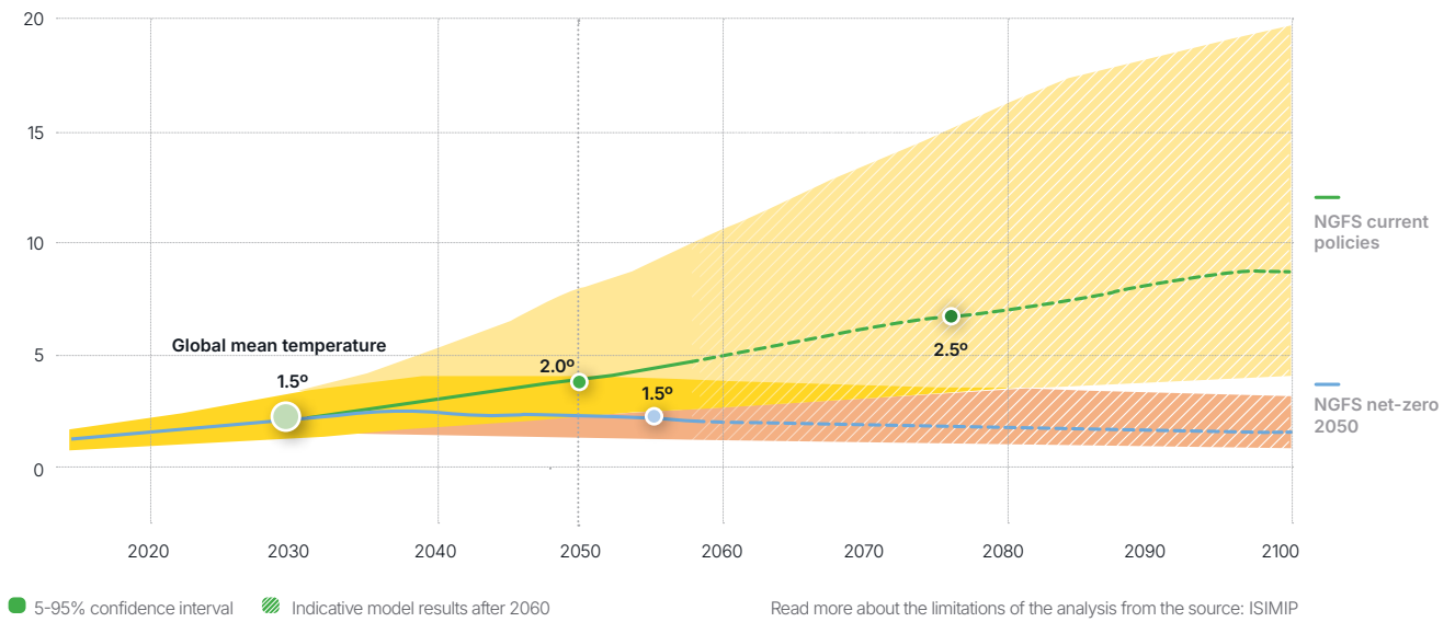
Figure 3. Number of days exposed to extreme heatwaves in Türkiye under different scenarios (HI > 40°C)
