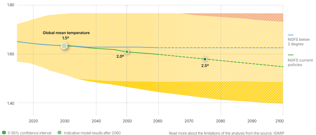
Figure 1. Long-term change in average daily precipitation in Türkiye under different scenarios
