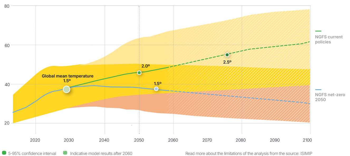
Figure 4. Number of days with weather conditions conducive to forest fires in Türkiye under different scenarios
