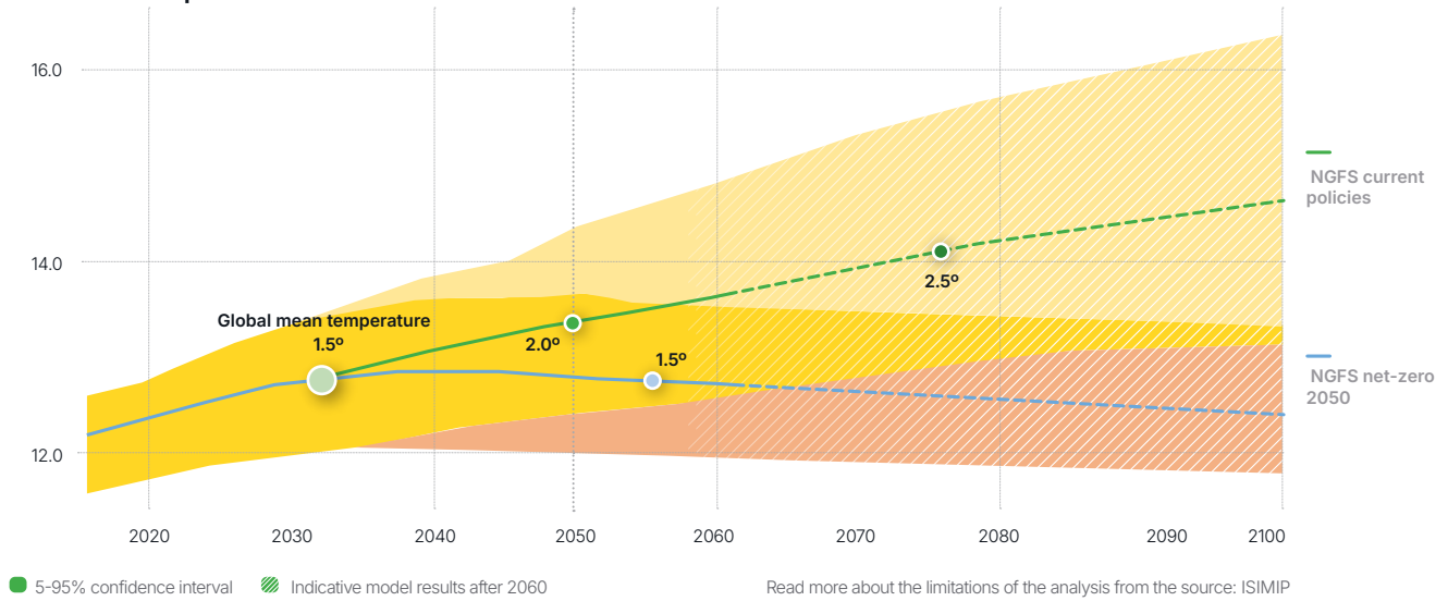
Figure 5. Long-term change in average air temperature in Türkiye under different scenarios
